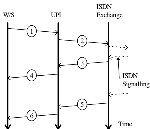
Figure 3. Message sequence: outgoing call from W/S
