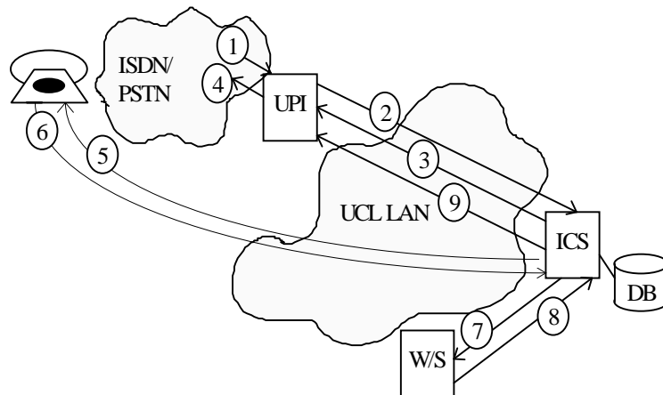
Figure 4. Incoming call handling
