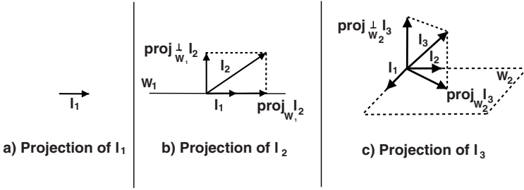
Fig. 4. Gram-Schmidt Process
